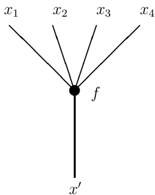
8. An operation f with profile (x_1, x_2, x_3, x_4, x')
