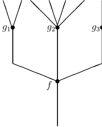
9. An operation f \circ (g_1, \dots, g_k) of P \circ Q , where k = 3
