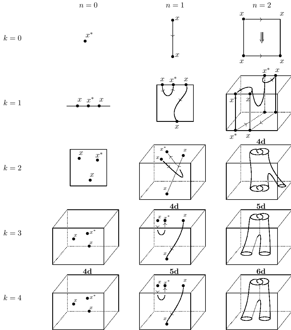
Figure 1: Examples of n -dimensional tangles in (n + k) -dimensional space.
