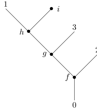
(c) The morphism \epsilon_{FUO} sends the operation in Figure 1(a) to the tree obtained by grafting the vertex labels.
