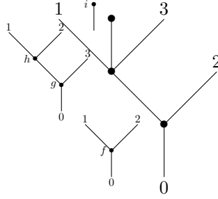
(a) An operation in FUFU(O)_3 .
