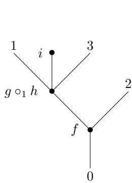
(b) The morphism FU\epsilon_O sends the operation in Figure 1(a) to the O -tree obtained by applying \epsilon_O to the vertex labels.
