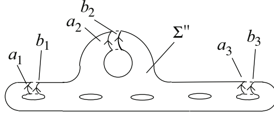
Figure 2. Surface \Sigma'' \subset \Sigma with oriented boundary curves a_i, b_i .
