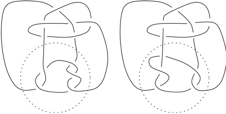
FIGURE 1. The Conway knot and the Kinoshita–Terasaka knot.
