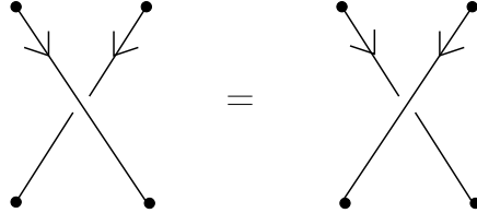
13. Tangle equation corresponding to symmetry
