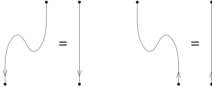
7. Tangle equations corresponding to the definition of adjunction
