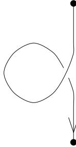
11. Tangle corresponding to the balancing b: x \rightarrow x
