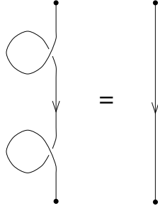
12. Tangle equation corresponding to unitarity of the balancing
