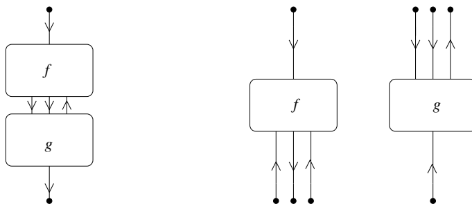
4. Composition and tensor product of tangles
