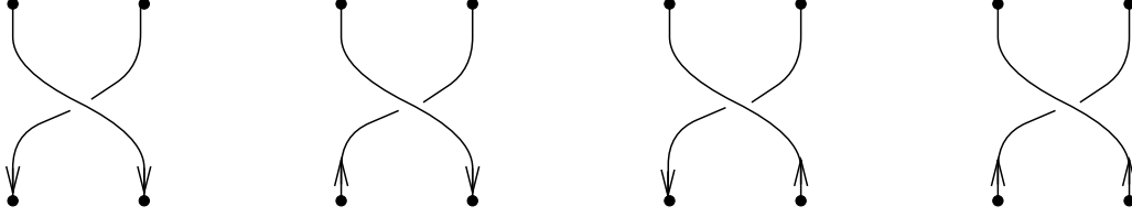
10. Tangles corresponding to B_{x,x}^{-1} , B_{x^*,x}^{-1} , B_{x,x^*}^{-1} , and B_{x^*,x^*}^{-1}
