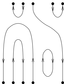
3. Typical tangle in 2 dimensions
