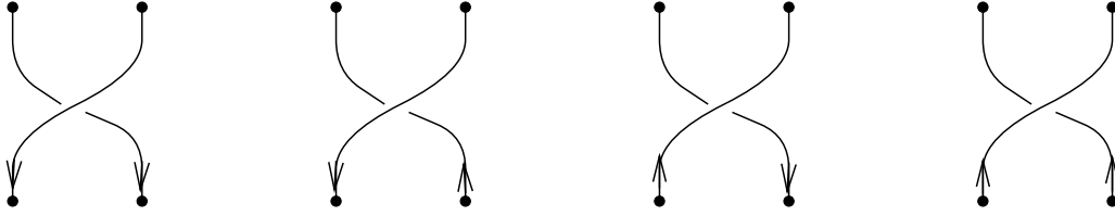
9. Tangles corresponding to B_{x,x} , B_{x^*,x} , B_{x,x^*} , and B_{x^*,x^*}
