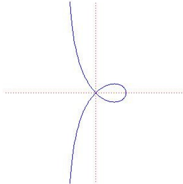
Right Strophoid
