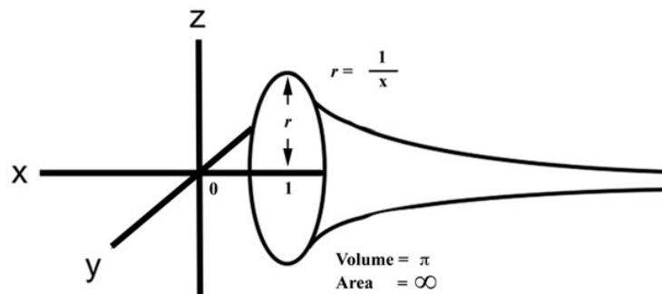
Torricelli's Trumpet
