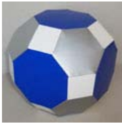
8. Truncated cuboctahedron
